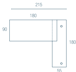
Desks with storage unit
