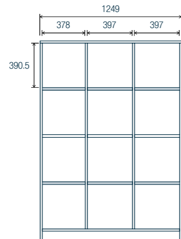
12 compartments
