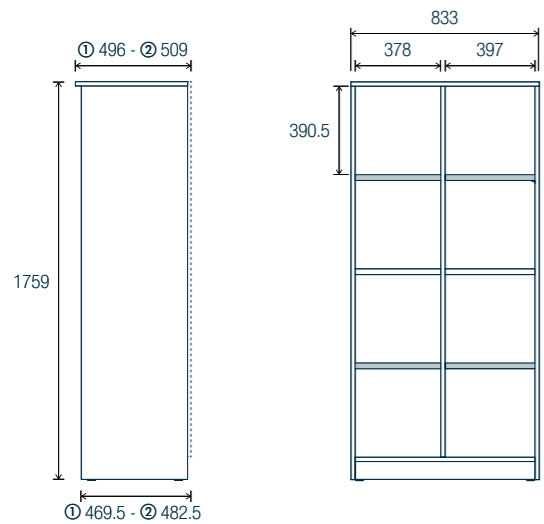
8 compartments
