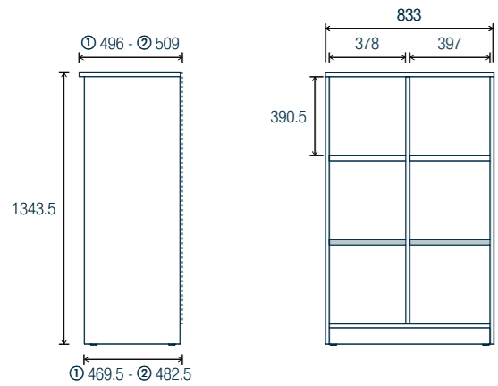
6 compartments
