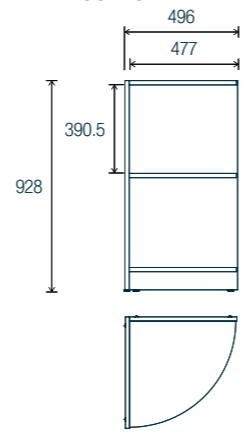
2-compartment corner
