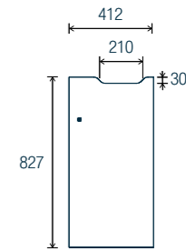
For 2 compartments
