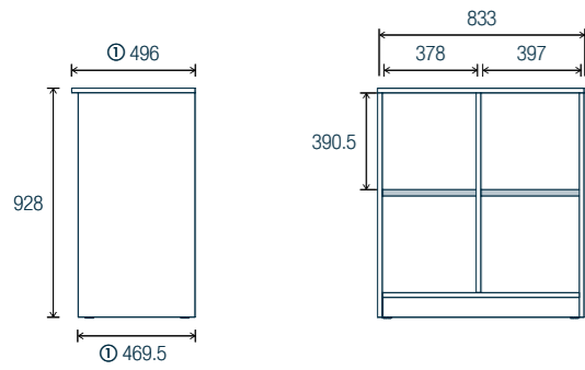
4 compartments
