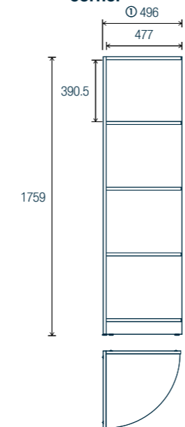
4-compartment corner
